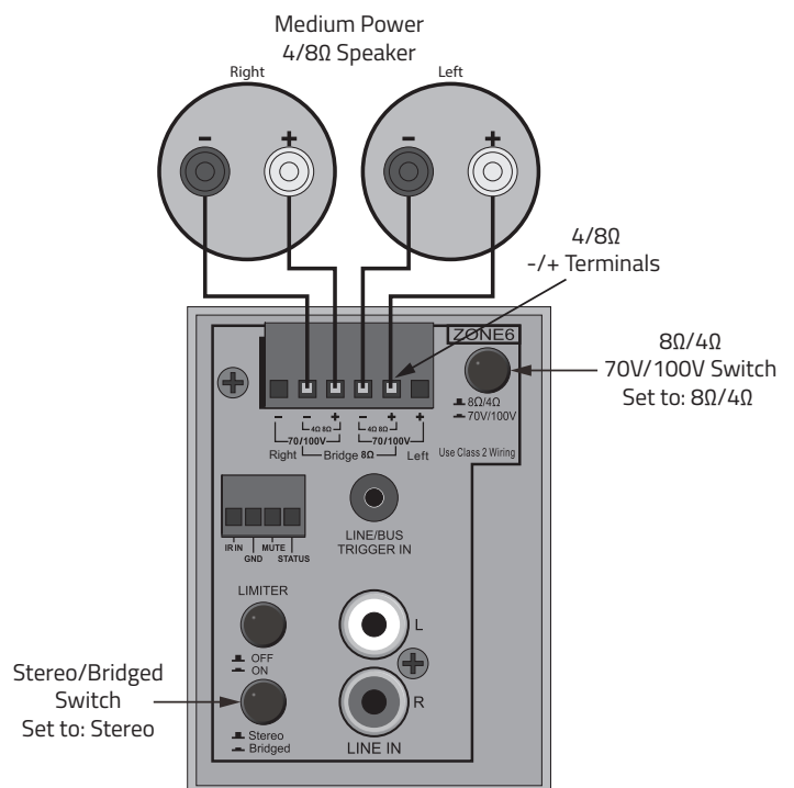
Stereo 4/8Ω Connection
