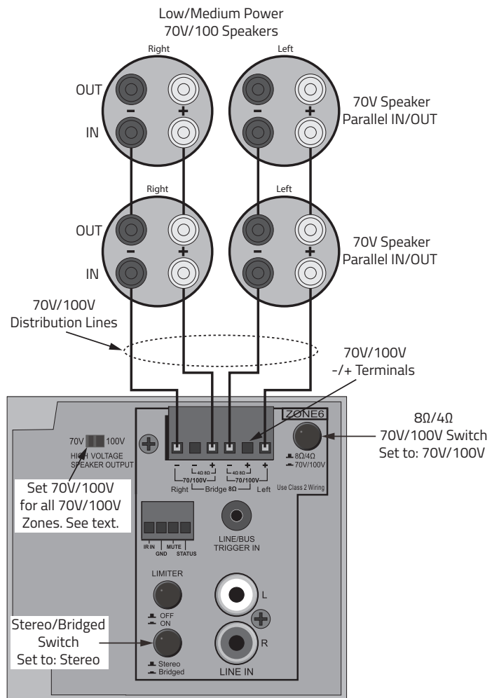
70V/100V Connection
