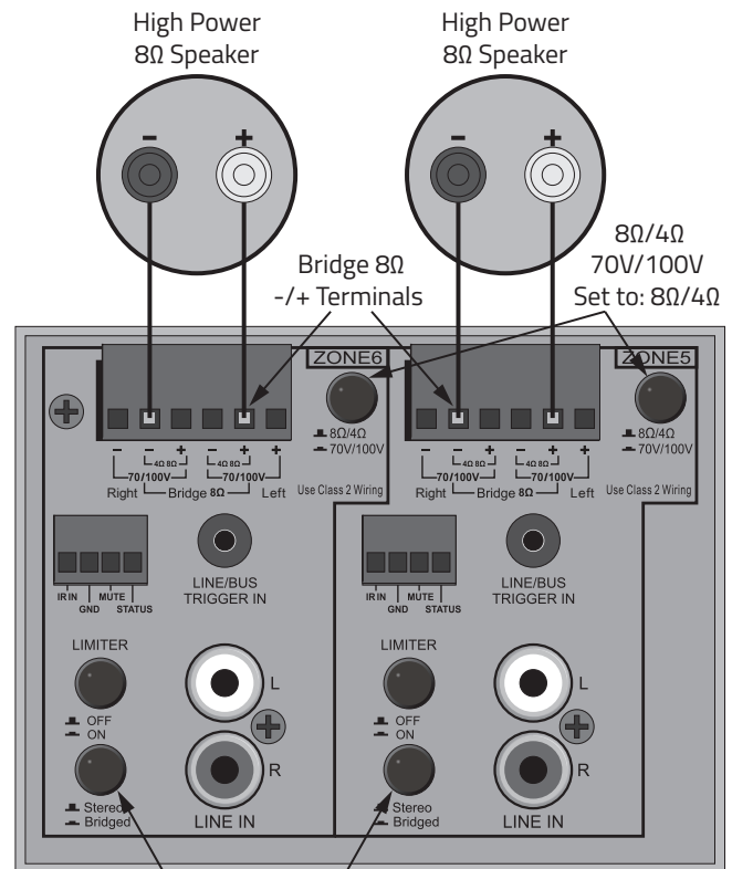
Stereo/Bridged Set to: Bridged Bridged 8Ω Connection
